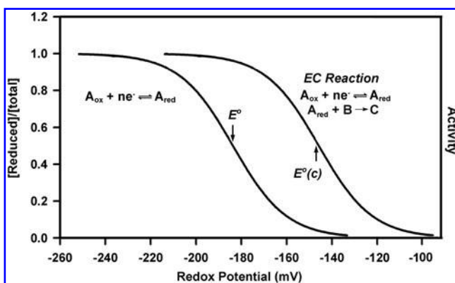
FIG. 1. Comparison of standard redox reactions (left) and an EC reaction (right) in which a redox process is coupled to a chemical reaction. B binds to (or reacts with) only the A_{\text{red}} state. Because only the reduced form of the protein can bind ligand, the apparent redox potential of the E_{\text{ox}}/E_{\text{red}} couple shifts to a more positive value.
